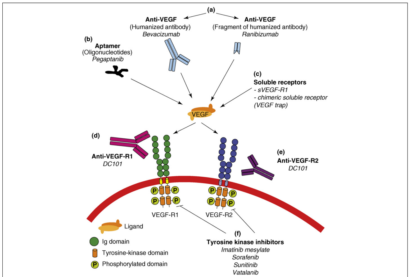
Figure 2. Anti-VEGF strategies currently used. Inhibition of VEGF signaling can be achieved with extracellular or intracellular inhibitors: (a) Monoclonal antibodies that target VEGF-A; (b) Oligonucleotides (aptamers) that bind the heparin-binding domain of VEGF165; (c) Chimeric soluble receptors (VEGF trap, a domain of VEGF-R1 and a domain of VEGF-R2 fused to the Fc fragment of an antibody) or the alternative spliced soluble form of VEGF-R1 (sVEGF-R1, or sflt-1); (d) Monoclonal antibodies that target VEGF-R1; (e) Monoclonal antibodies that target VEGF-R2; (f) Small-molecule VEGF-receptor tyrosine kinase inhibitors that block ligand-dependent receptor autophosphorylation. In addition, antisens and siRNA strategies that target VEGF or VEGF receptors are under development (not shown).
